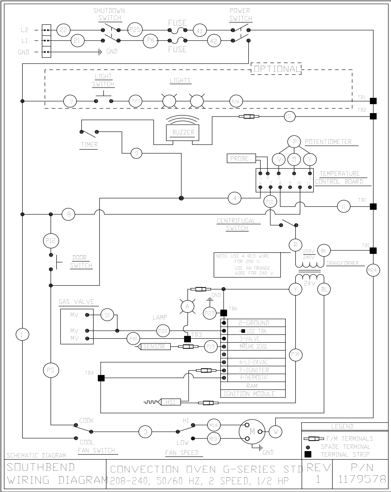
Wiring Diagram for 208-240 Volt Models with Standard Controls
