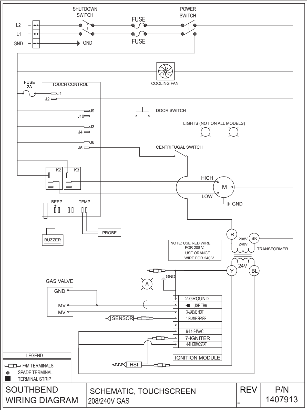
Wiring Diagram for 208-240 Volt Models with Touchscreen Controls
